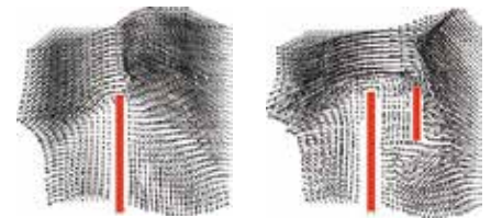
標準大型広幅断面 Cross section of standard large wide blade MR205 二重翼断面 Cross section of double-blade structure of MR205 impeller
